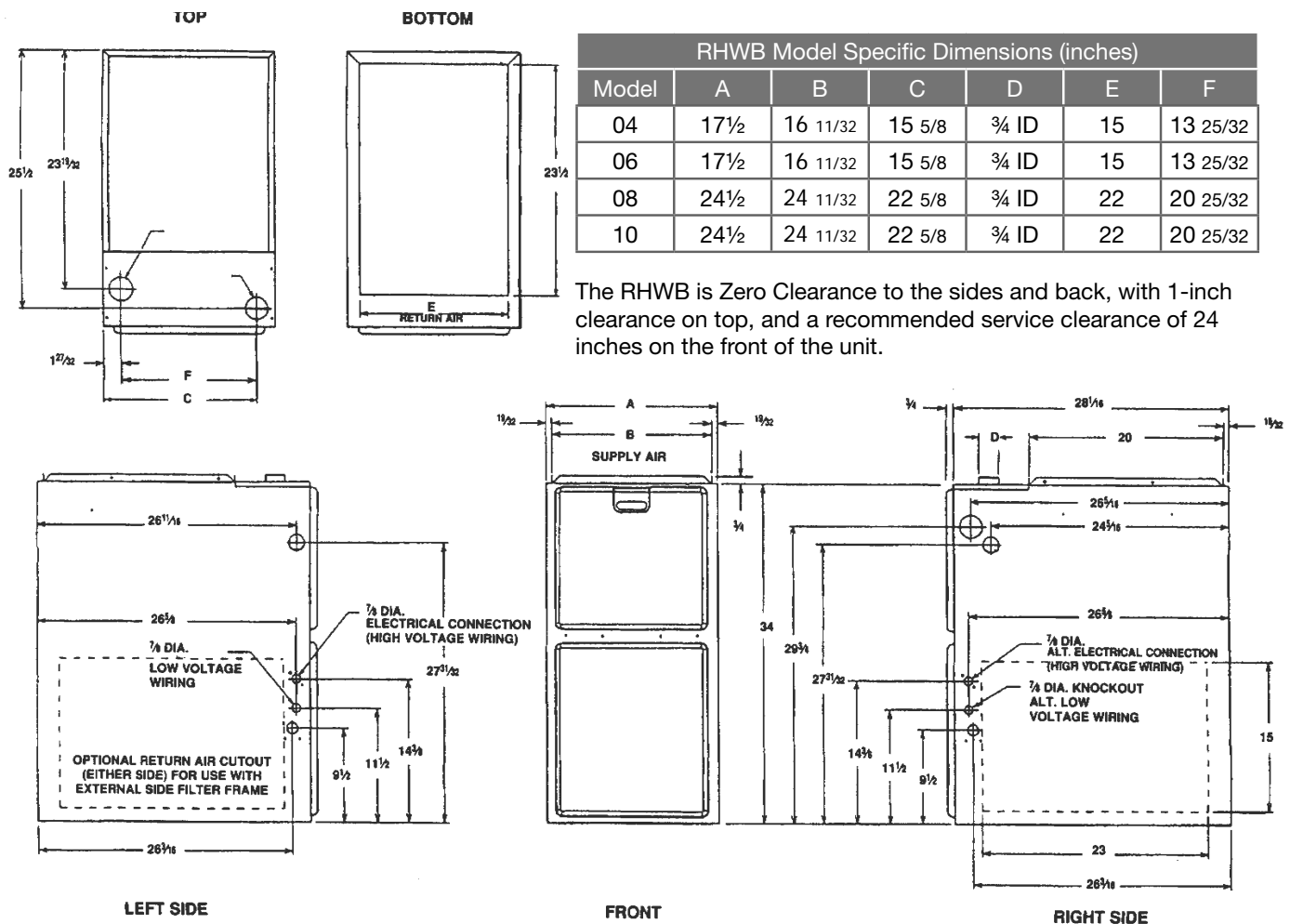
Figure 11 - RHWB Dimensions and Clearances
