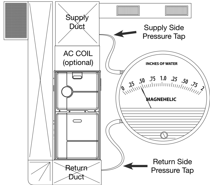
Figure 10 - Magnehelic Gauge Pressure Test
