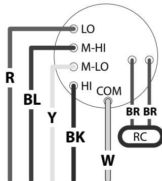
Figure 7 - Hydronic Air Handler Motor Wire Colors
