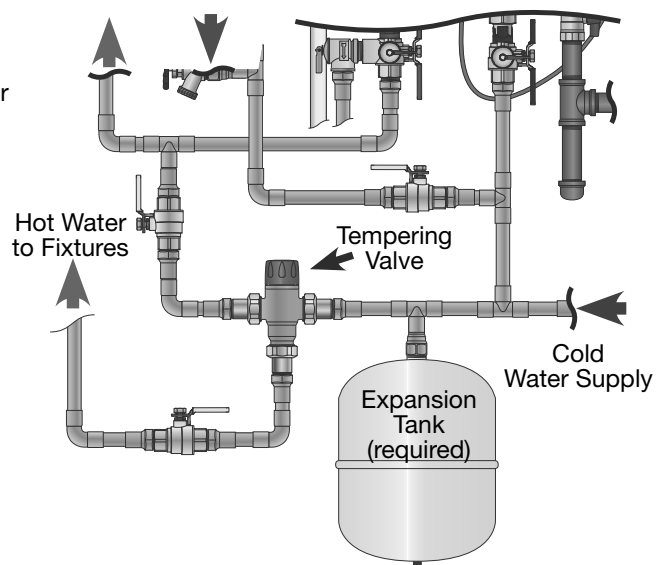
Figure 4 - Tempering Valve and Expansion Tank
