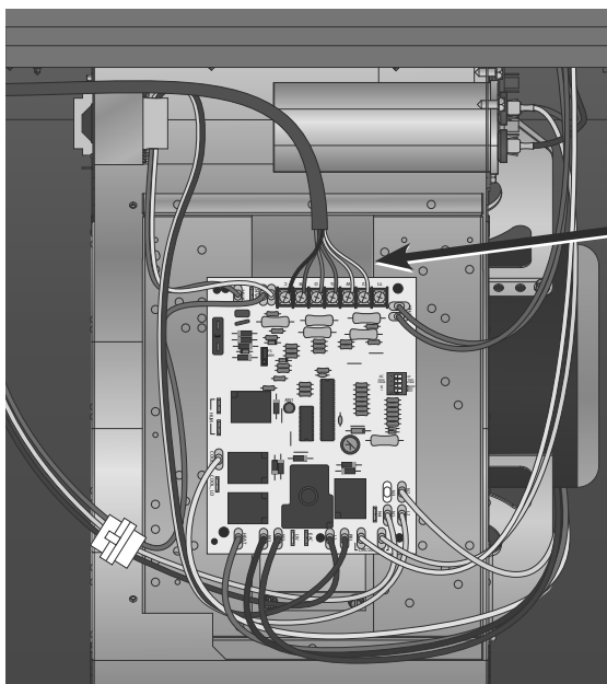
Figure 9 - Room Thermostat Connection
