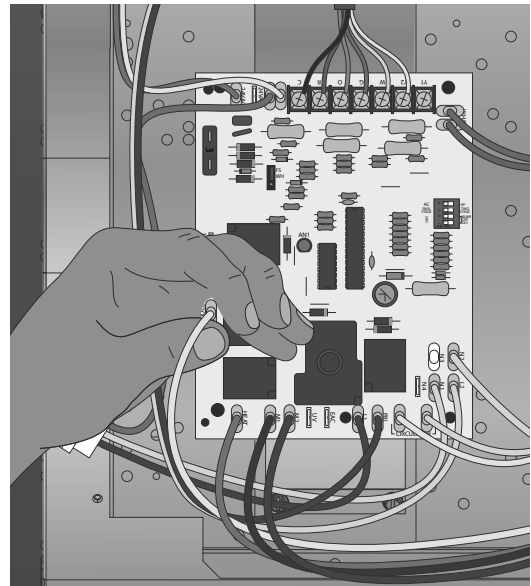
Figure 8 - Connecting Fan Speed wires
