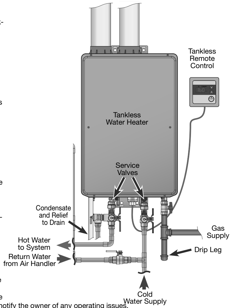
Figure 5 - Tankless Water Heater
